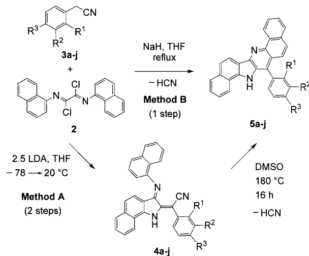
Scheme 5. Synthesis of 15 H -benzo[ h ]benzo[6,7]indolo[3,2- b ]quinolines 5
