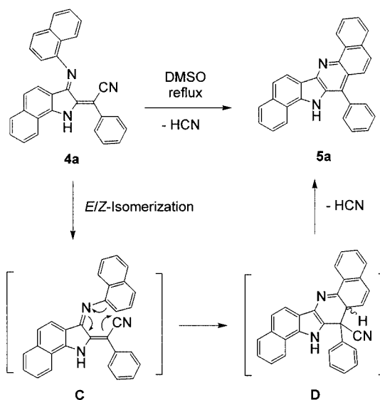
Scheme 4. Synthesis of 5a by electrocyclicization of 4a
