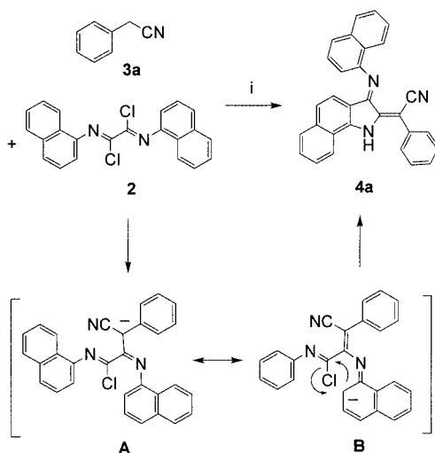
Scheme 3. Synthesis of 2-alkylidene-3-iminobenzindole 4a ; i : 1) 2.5 equiv. LDA, THF, 0 °C, 2) 2 , -78 → 20 °C
