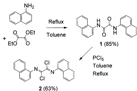
Scheme 2. Synthesis of N,N' -bis(1-naphthyl)oxaldiimidoyl dichloride
