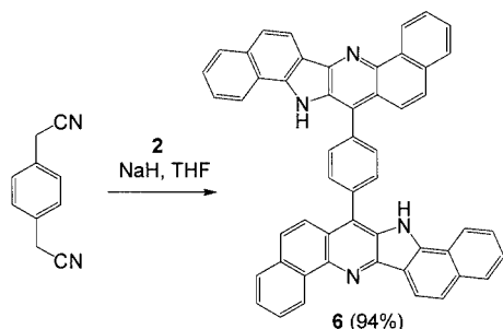
Scheme 6. Cyclization of 1,4-bis(cyanomethyl)benzene with 2
