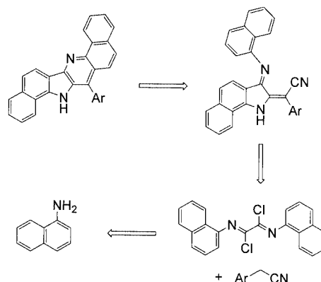
Scheme 1. Retrosynthetic analysis
